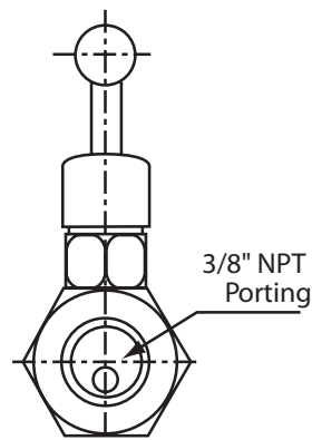
PORT "B"
