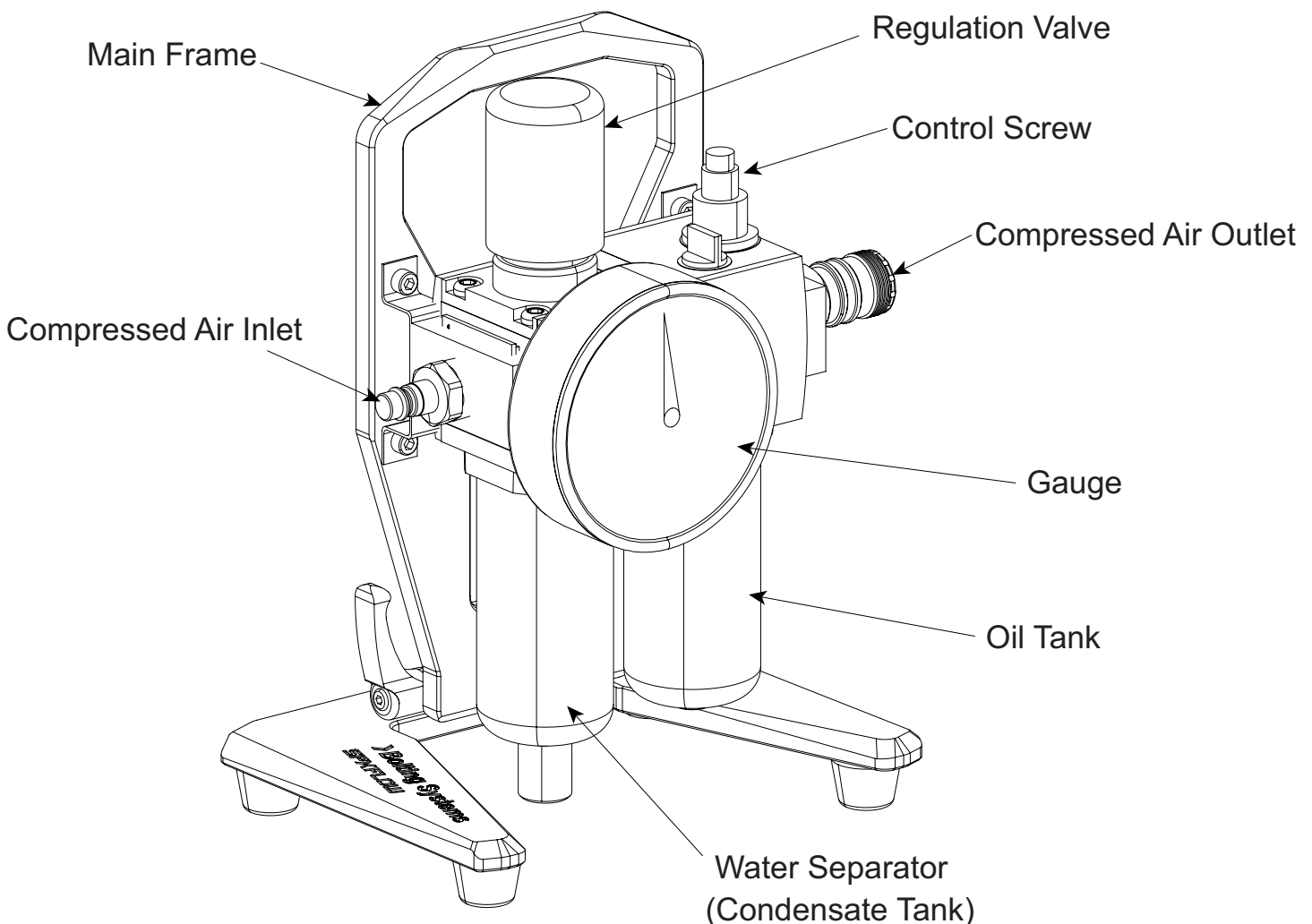
Fig. 2.6 Air Control Unit
