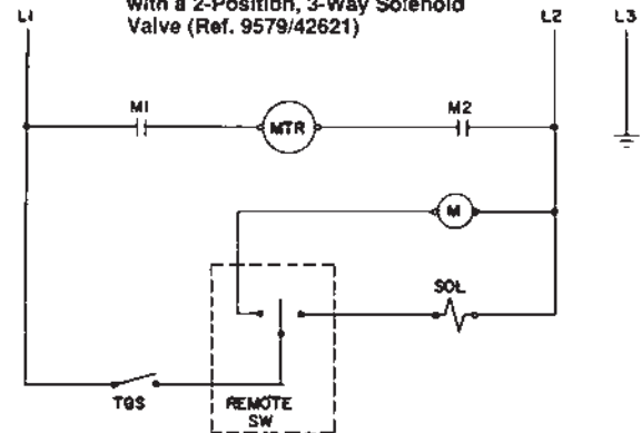
Electrical Schematic for Units with a 2 Position, 4-Way Solenoid Valve (Ref. 9582/61084)
