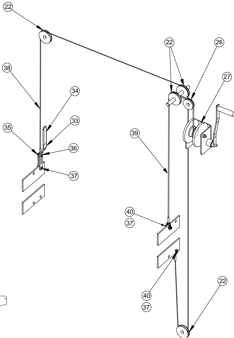
CABLE DIAGRAM
