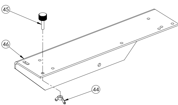
MOUNTING BRACKET for P159 and 4016 HAND PUMP
