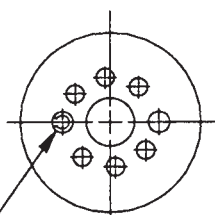
ROTOR TOP VIEW ROLL PIN LOCATION (POSITION OPENING AS SHOWN)
