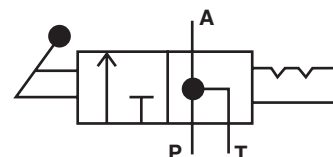
J.I.C. SYMBOL
