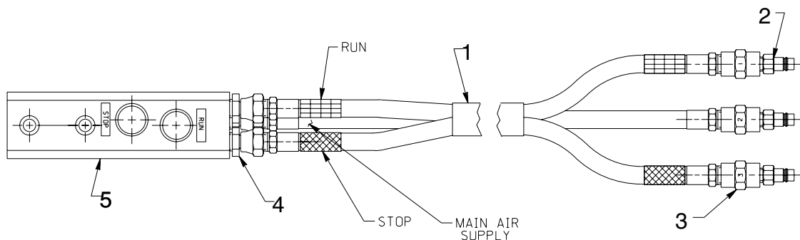
HAND CONTROL CONNECTIONS
