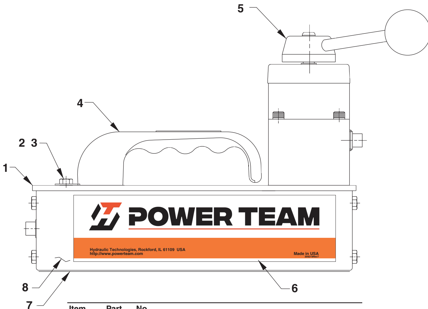
SIDE VIEW
