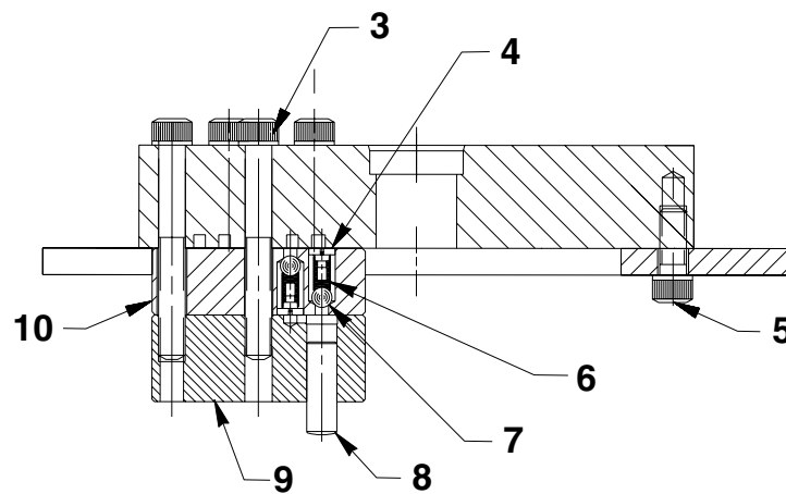
SECTION "Z-Z"
