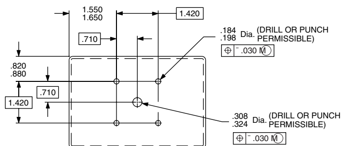
Mounting Hole Detail (Cover and Gasket for Item 6)
