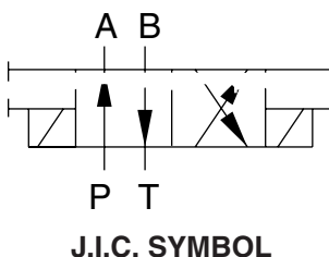
J.I.C. SYMBOL
