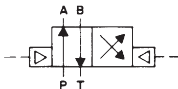
J.I.C. SYMBOL
