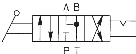
HYDRAULIC SCHEMATIC
