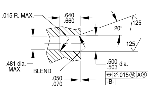
PORT DETAIL
