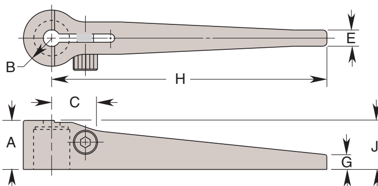
Swing Clamp Arm
