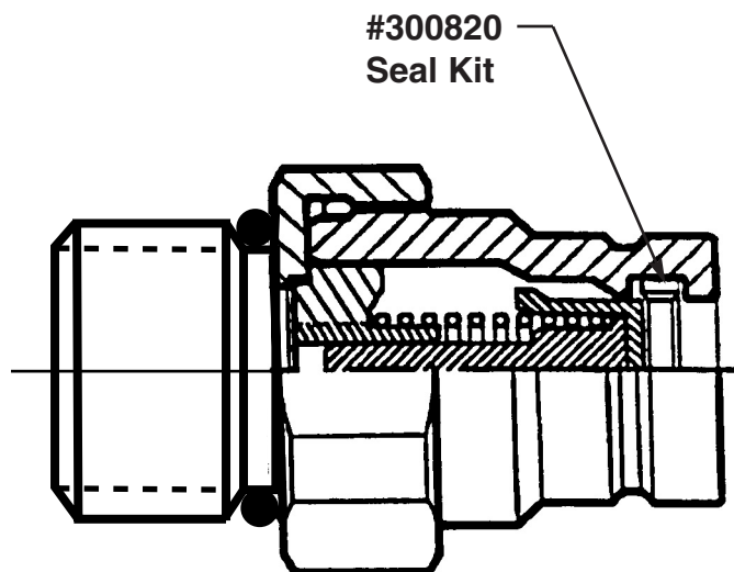
Coupler (With seal installed)
